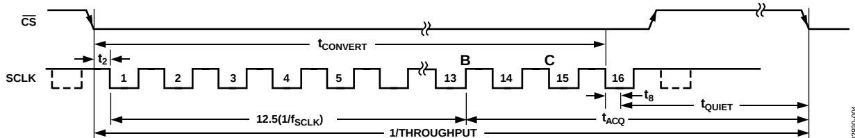
Figure 4. Serial Interface Timing Example
