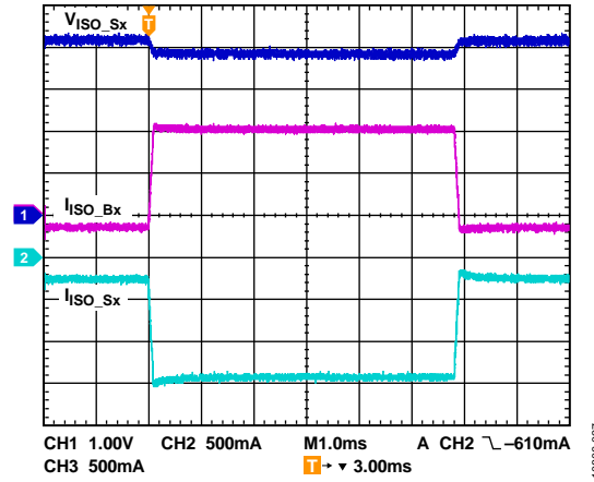
Figure 27. Load Transient, I_{ISO\_Sx} Load = 300 mA to 1500 mA to 300 mA, EN\_CHG = \text{High} , ILIM[3:0] = 0110 (Binary) = 500 mA
