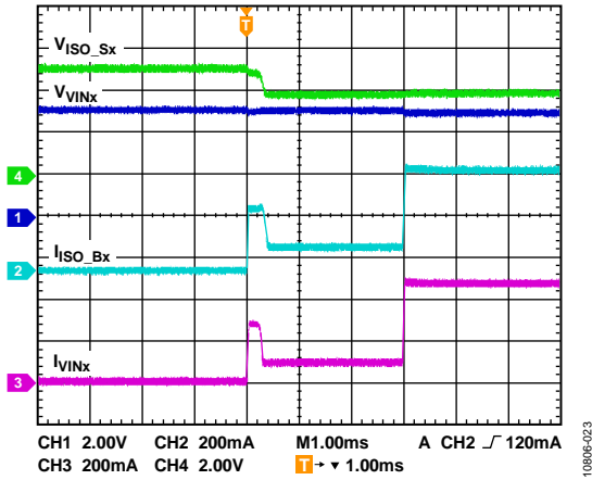
Figure 23. Charging Startup, V_{VINx} = 5.0\text{ V} , ILIM[3:0] = 0110 (Binary) = 500 mA, ICHG[4:0] = 01110 (Binary) = 750 mA
