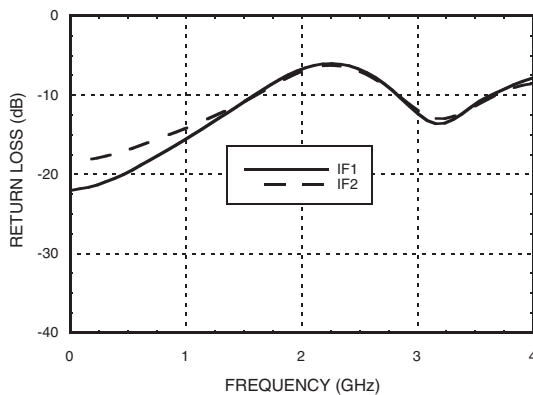
IF Return Loss [1]
