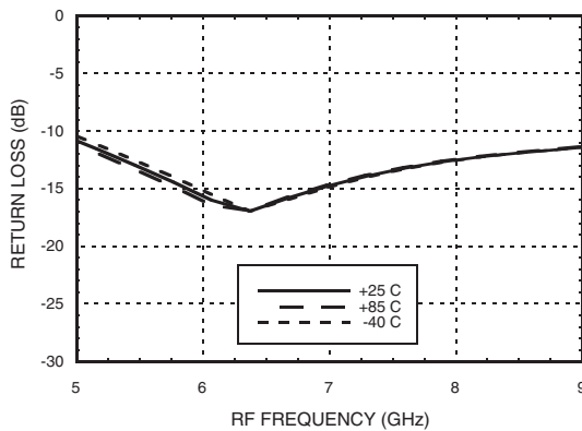
RF Return Loss vs. Temperature
