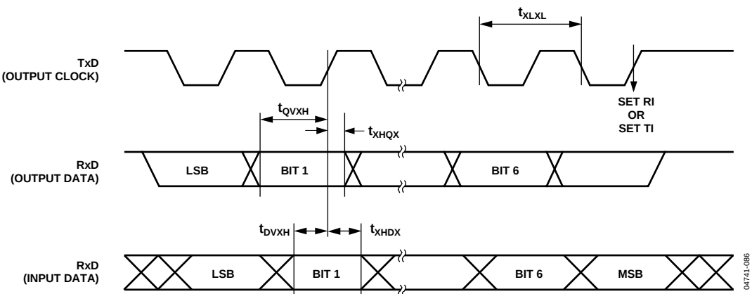
Figure 80. UART Timing in Shift Register Mode
