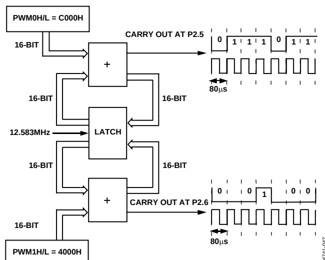
Figure 42. PWM Mode 4
