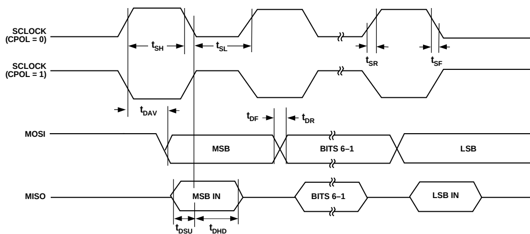
Figure 76. SPI Master Mode Timing (CHPA = 1)
