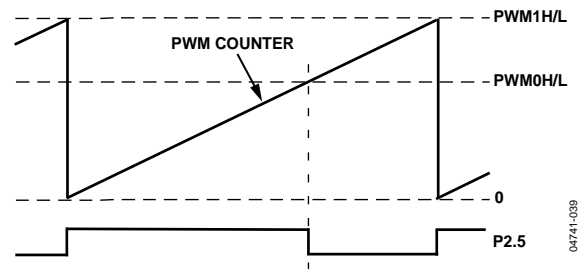
Figure 39. PWM in Mode 1
