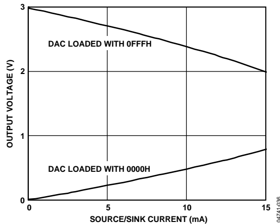
Figure 36. Source and Sink Current Capability with V_{REF} = AV_{DD} = 3\text{ V}
