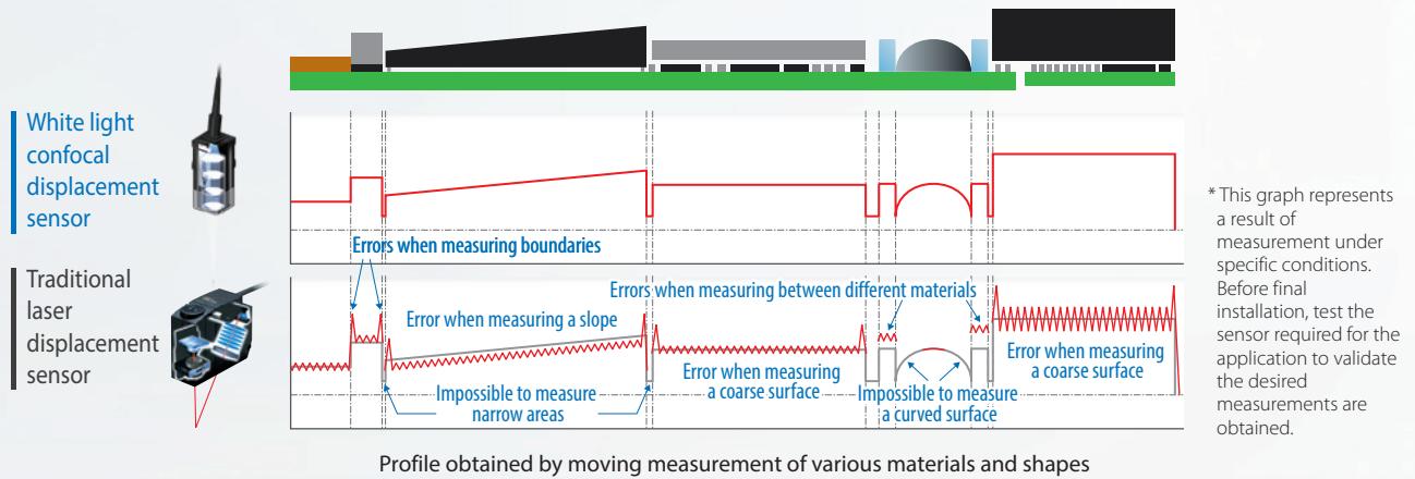
Profile obtained by moving measurement of various materials and shapes
