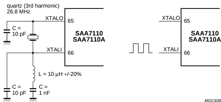
a. with quartz crystal. b. with external clock.
