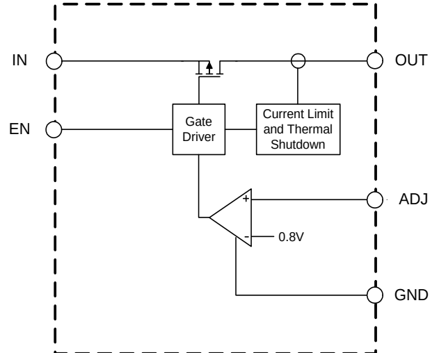
Adjustable Version
