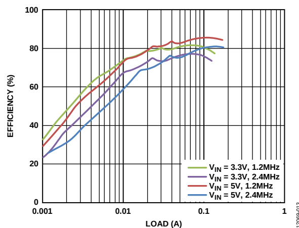
Figure 14. Inverting Regulator Efficiency vs. Current Load, V_{NEG} = -15V , T_A = 25^\circ C
