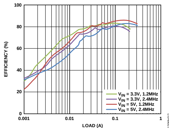
Figure 13. Inverting Regulator Efficiency vs. Current Load, V_{NEG} = -9V , T_A = 25^\circ C
