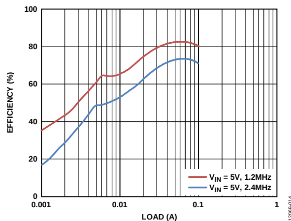
Figure 15. Inverting Regulator Efficiency vs. Current Load, V_{NEG} = -34V , T_A = 25^\circ C
