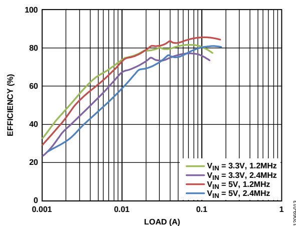
Figure 14. Inverting Regulator Efficiency vs. Current Load, V_{NEG} = -15\text{ V} , T_A = 25^\circ\text{C}
