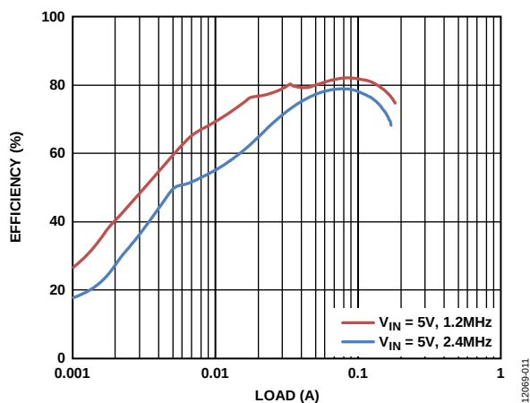
Figure 12. Boost Regulator Efficiency vs. Current Load, V_{POS} = 34\text{ V} , T_A = 25^\circ\text{C}
