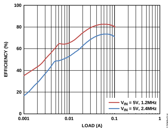
Figure 15. Inverting Regulator Efficiency vs. Current Load, V_{NEG} = -34\text{ V} , T_A = 25^\circ\text{C}
