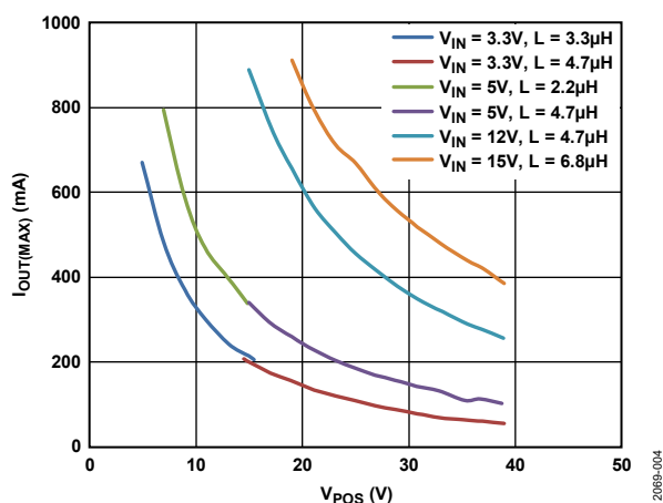
Figure 5. Boost Regulator Maximum Output Current, f_{SW} = 2.4 MHz, T_A = 25^\circ\text{C} , Based on Target of 70% I_{LIM(BOOST)}
