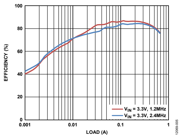
Figure 6. Boost Regulator Efficiency vs. Current Load, V_{IN} = 3.3 V, V_{POS} = 5 V, T_A = 25^\circ\text{C}
