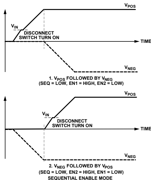
Figure 43. Sequential Enable Mode
