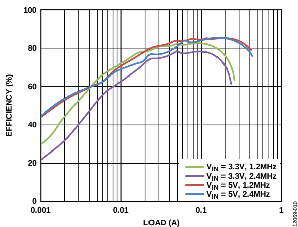
Figure 11. Boost Regulator Efficiency vs. Current Load, V_{POS} = 15\text{ V} , T_A = 25^\circ\text{C}
