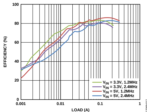
Figure 13. Inverting Regulator Efficiency vs. Current Load, V_{NEG} = -9\text{ V} , T_A = 25^\circ\text{C}
