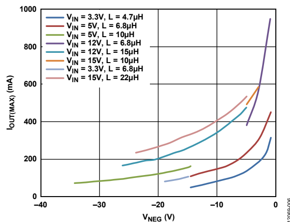
Figure 7. Inverting Regulator Maximum Output Current, f_{SW} = 1.2 MHz, T_A = 25^\circ\text{C} , Based on Target of 70% I_{LIM(INVERTER)}
