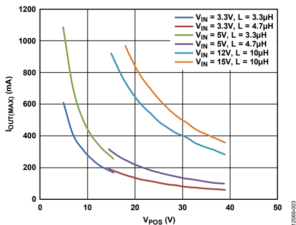
Figure 4. Boost Regulator Maximum Output Current, f_{SW} = 1.2 MHz, T_A = 25^\circ\text{C} , Based on Target of 70% I_{LIM(BOOST)}
