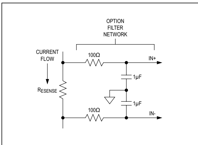
Figure 7. Filter Network
