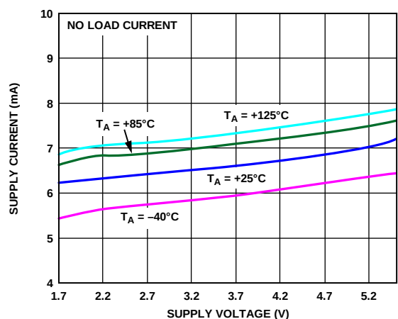
Figure 12. Quiescent Supply Current vs. Supply Voltage
