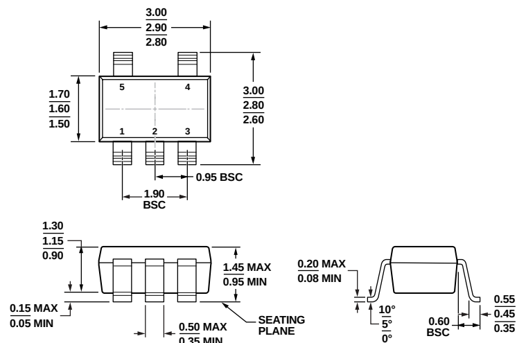
COMPLIANT TO JEDEC STANDARDS MO-178-AA Figure 32. 5-Lead Small Outline Transistor Package [SOT-23] (RJ-5) Dimensions shown in millimeters
