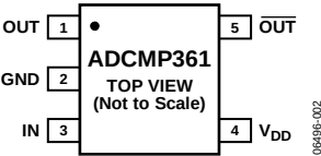
Figure 4. Pin Configuration
