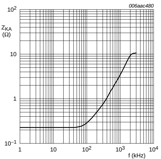
Fig 20. TL431XFTD: Dynamic cathode-anode impedance as a function of frequency; typical values
