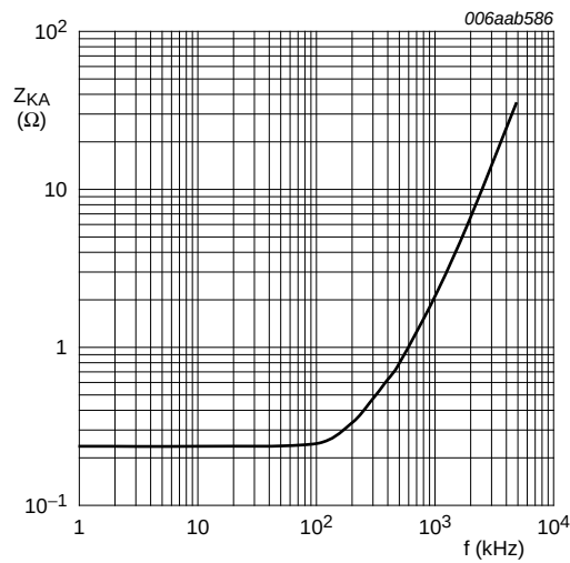
Fig 19. All types except TL431XFTD and TL431XSDT: Dynamic cathode-anode impedance as a function of frequency; typical values
