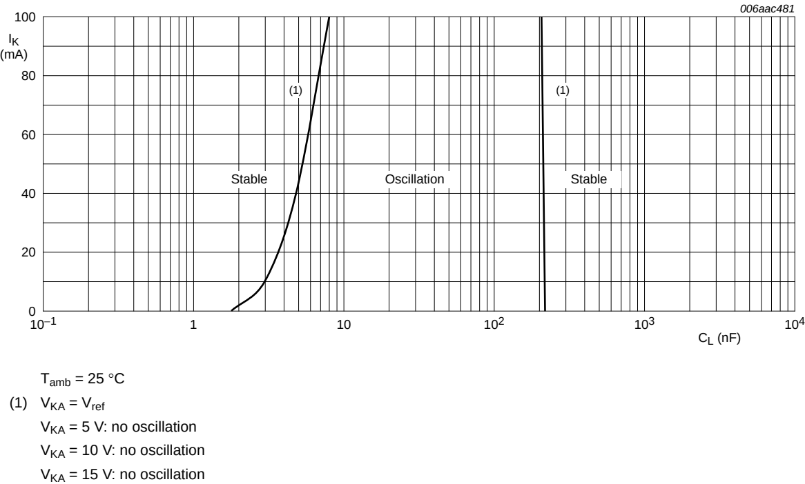
Fig 26. TL431XFDT: Cathode current as a function of load capacitance; typical values
