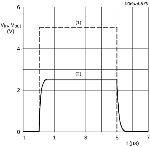
T_{amb} = 25\text{ }^{\circ}C (1) Input (2) Output
