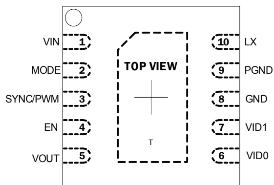
MLP10: 3X3 10 LEAD
