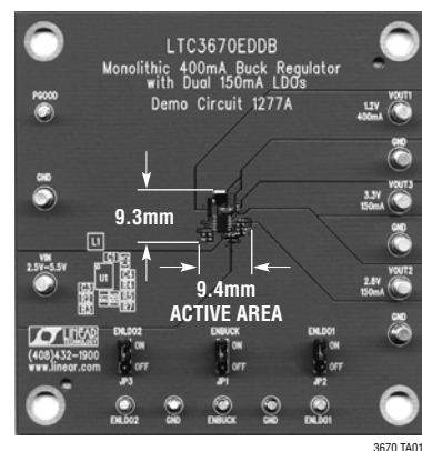
Demoboard
