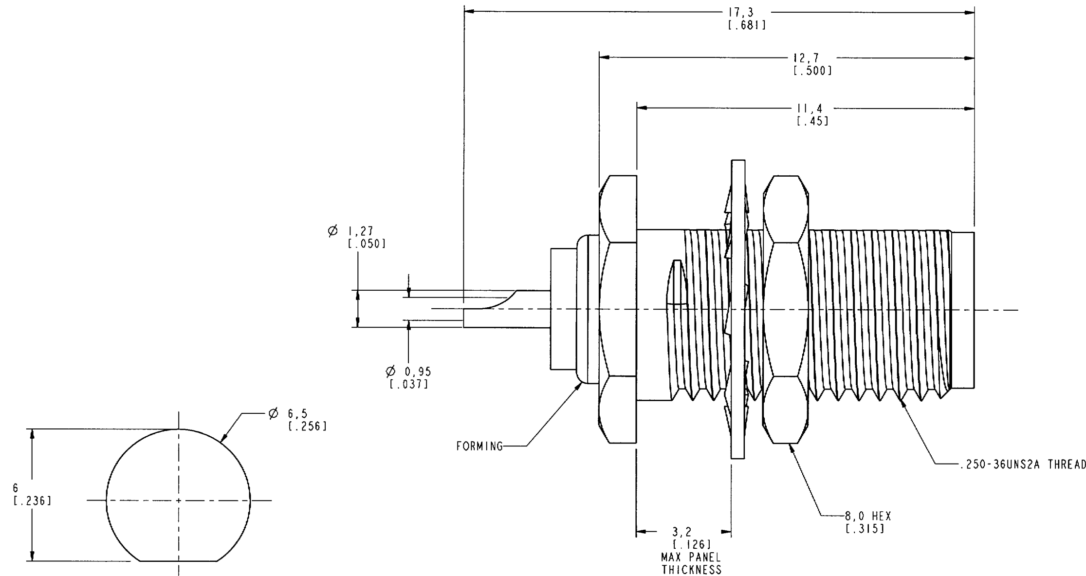
RECOMMENDED MOUNTING HOLE DIMENSIONS SCALE 6.000
