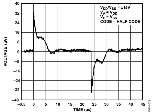
Figure 53. Digital Feedthrough
