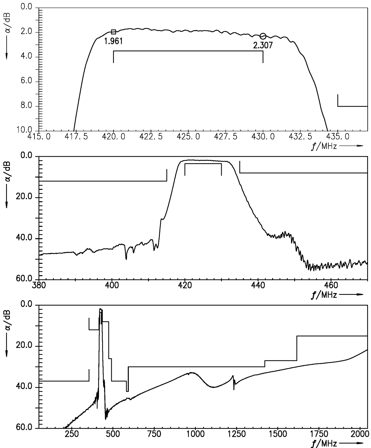
Figure 4: Attenuation.
