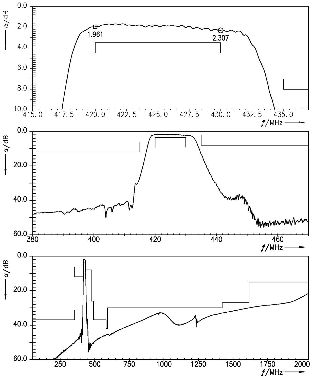
Figure 4: Attenuation.
