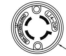
FACE VIEW OF MALE INSERT
