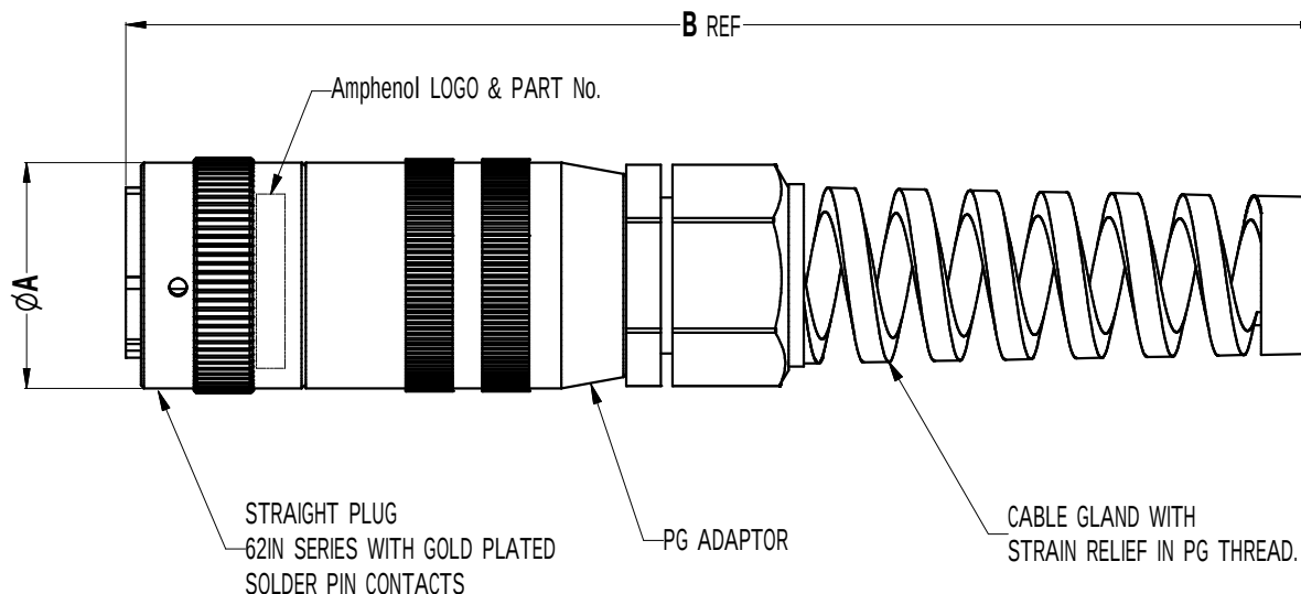
Parts List, Dimensions in mm
