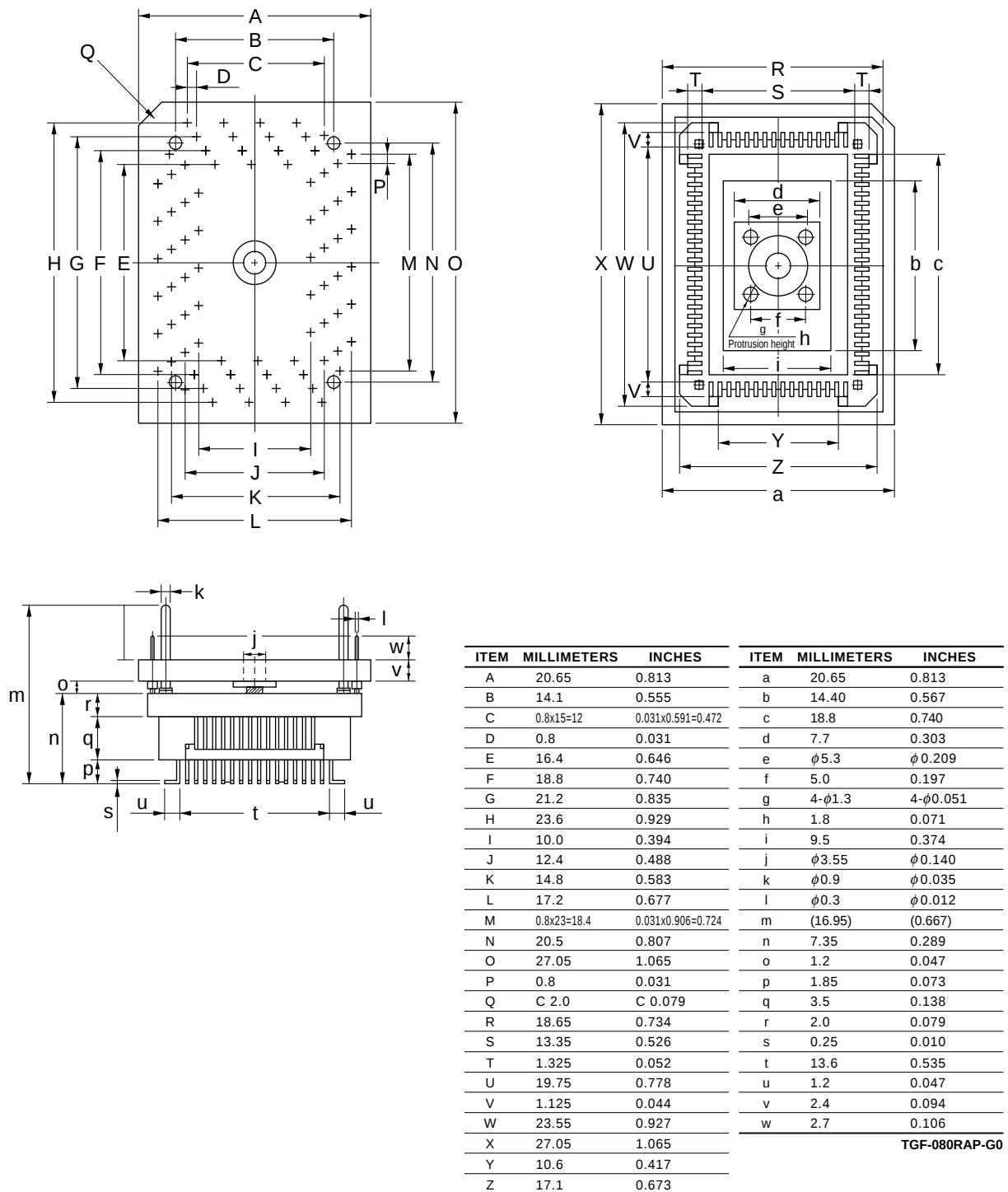
Figure A-2. Dimensions of TGF-080RAP (Reference)
