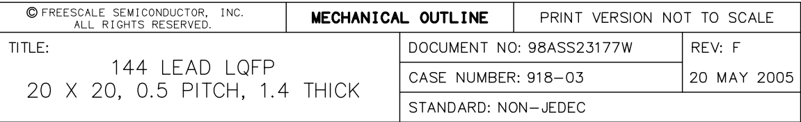
Figure 51. LQFP144 mechanical drawing (Part 2 of 3)
