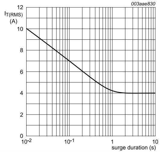
f = 50 Hz; T_{mb} \leq 107\text{ }^{\circ}\text{C} Fig. 2. RMS on-state current as a function of surge duration; maximum values
