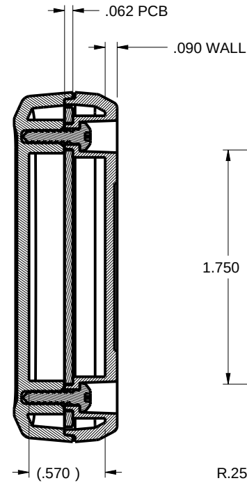
SECTION B-B
