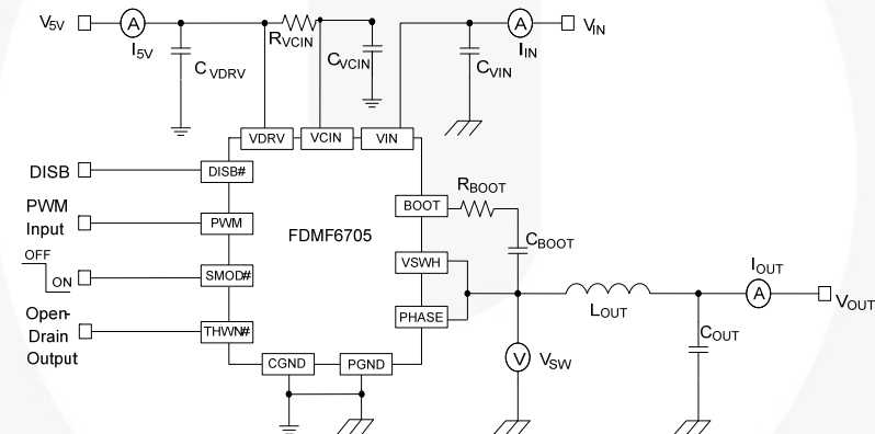
Figure 28. Power Loss Measurement Block Diagram
