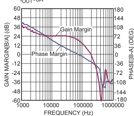
Bode Plot I_{OUT} = 8A
