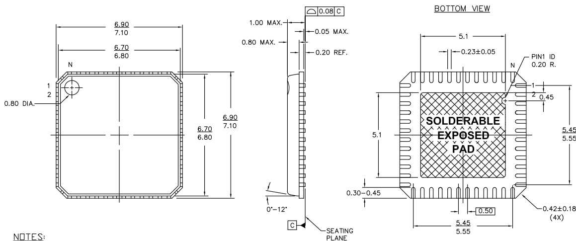
BOTTOM VIEW
