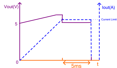
Figure 6: Over-Current Limit
