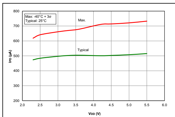
FIGURE 31-50: I_{PO} , Comparator, NP Mode ( CxSP = 1 ), PIC16F1782/3 Only.
