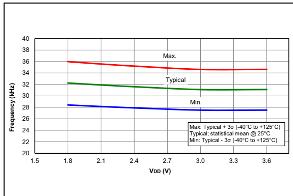
FIGURE 31-57: LFINTOSC Frequency, PIC16F1782/3 Only.
