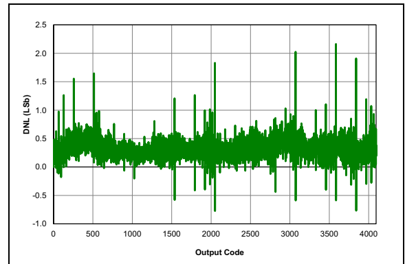
FIGURE 31-94: ADC 12-bit Mode, Single-Ended DNL, V_{DD} = 5.5V , T_{AD} = 4\text{ }\mu\text{S} , 25^\circ\text{C} .
