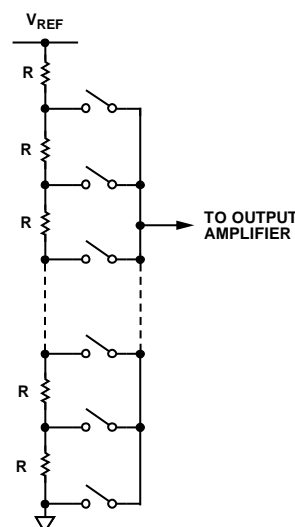
Figure 47. Resistor String Structure
