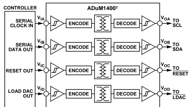
Figure 60. Isolated Interface
