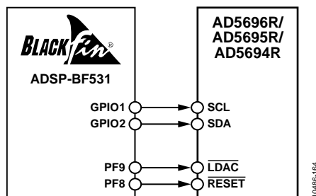
Figure 58. ADSP-BF531 Interface
