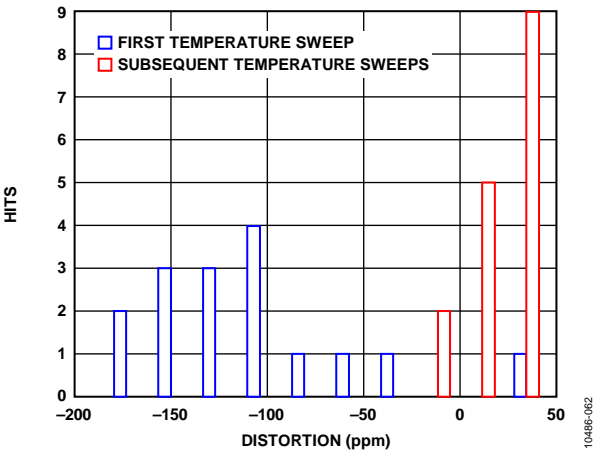
Figure 57. Thermal Hysteresis
