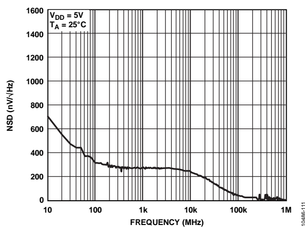
Figure 9. Internal Reference Noise Spectral Density vs. Frequency
