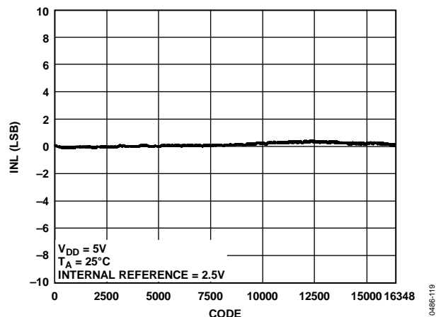
Figure 14. AD5695R INL
