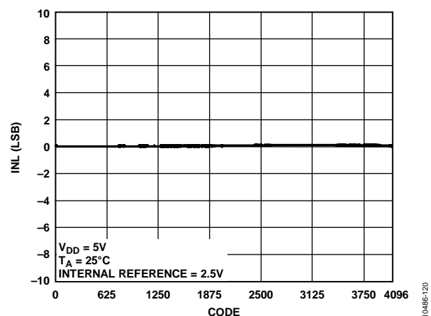
Figure 15. AD5694R INL
