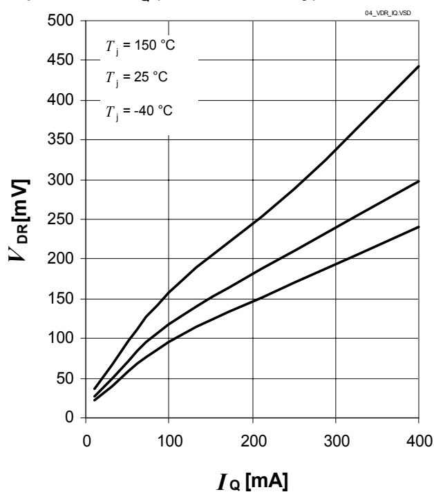
Dropout Voltage V_{dr} versus Output Current I_Q (5 V versions only)
