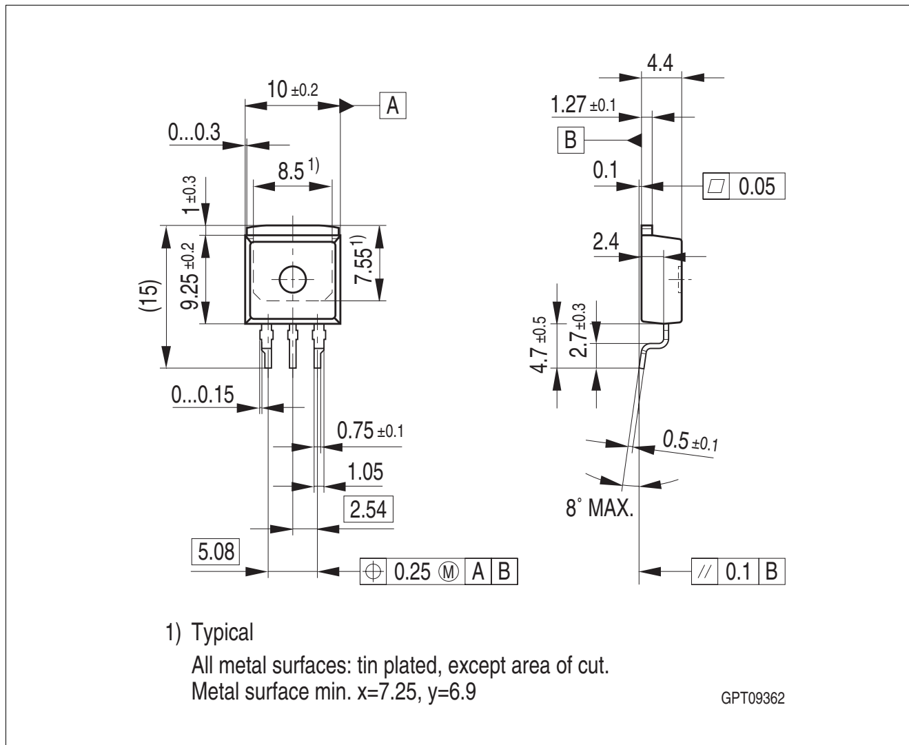
Figure 5 PG-TO263-3
