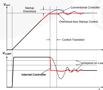
Figure 37. Startup without Overshoot
