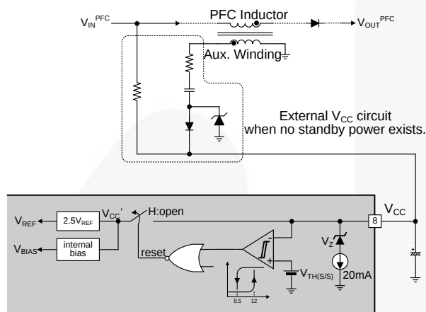
Figure 23. Startup Circuit
