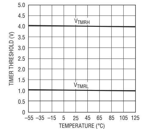
TIMER Threshold vs Temperature
