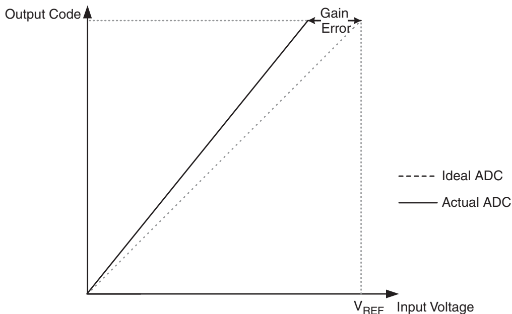
Figure 13-10. Gain Error
