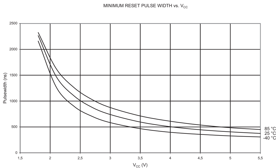
Figure 17-52. Minimum Reset Pulse Width vs. V_{CC}
