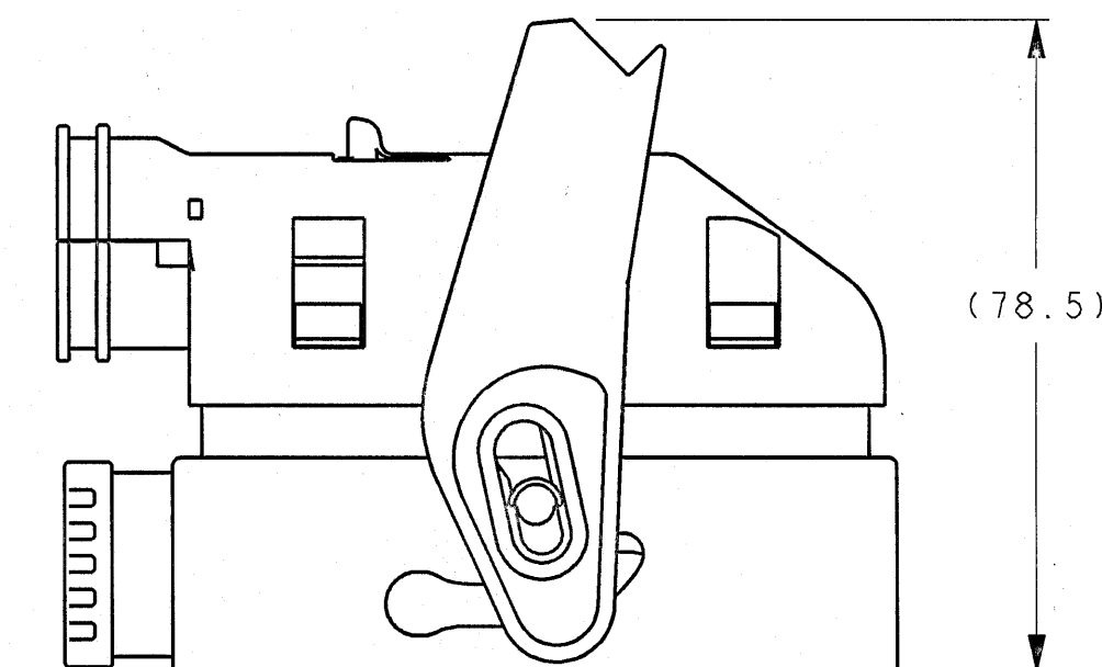
ASSEMBLY AT HIGHEST LOCATION DURING INSTALLATION
