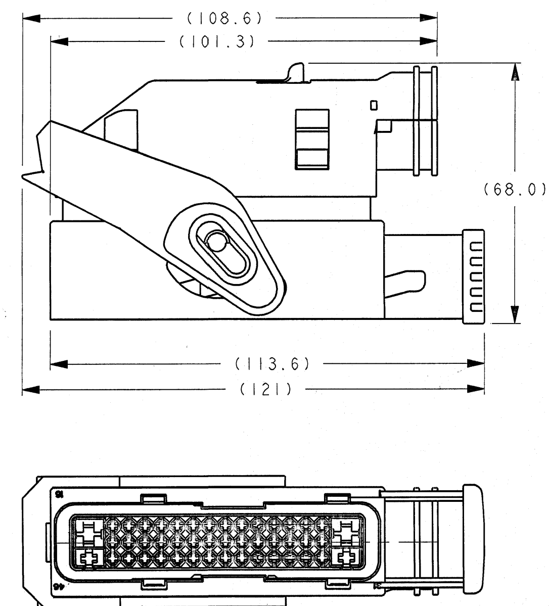
OPEN CONDITION: RIGHT HAND VERSION COVER SHIPPED SEPARATELY COVER SHOWN FOR VISUALIZATION ONLY LEFT HAND VERSION SYMMETRICALLY OPPOSITE
