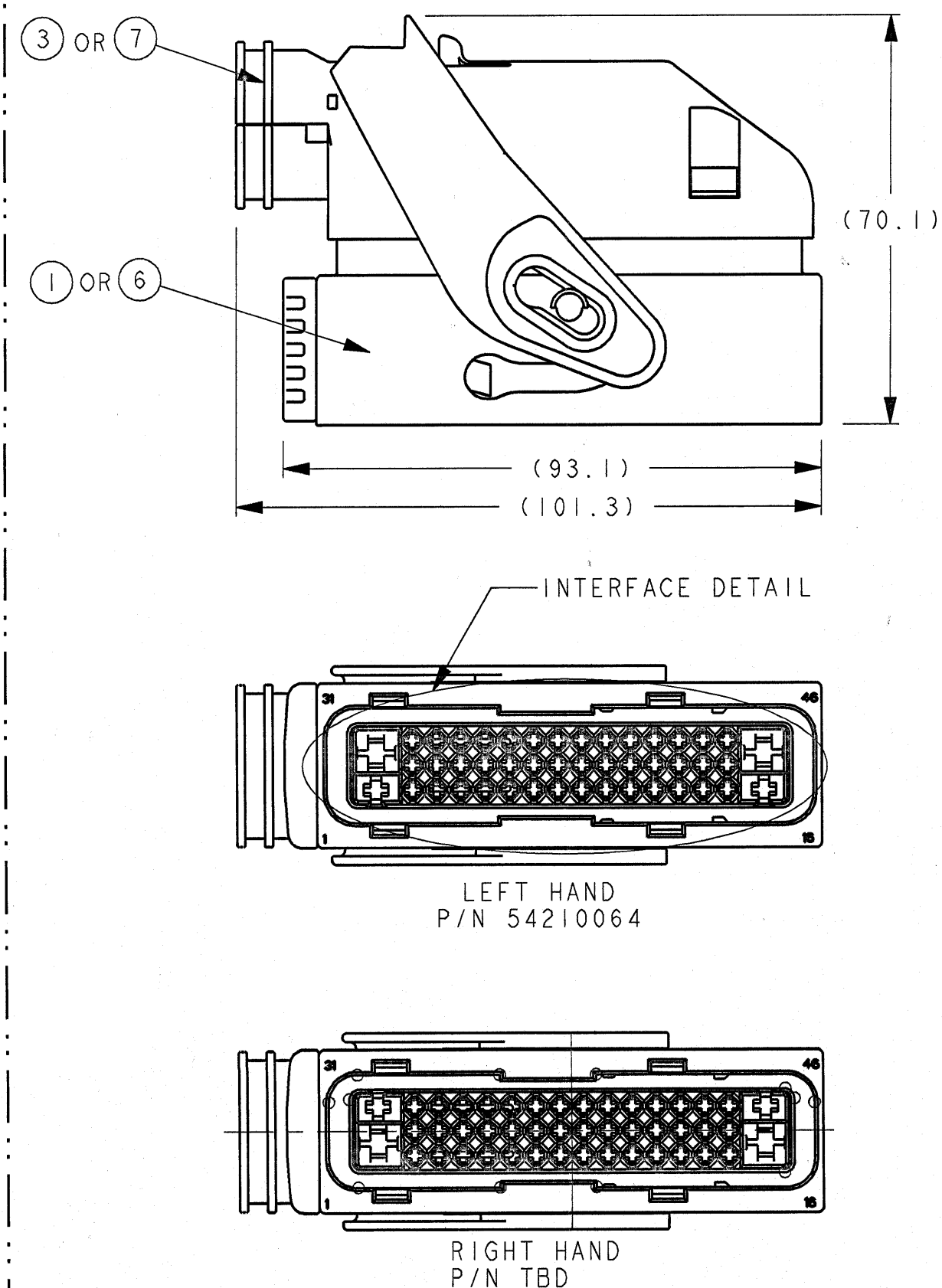
INSTALLATION OVERALL DIMENSIONS: CLOSED POSITION
