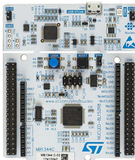
Top view of the NUCLEO-8L152R8 board.
