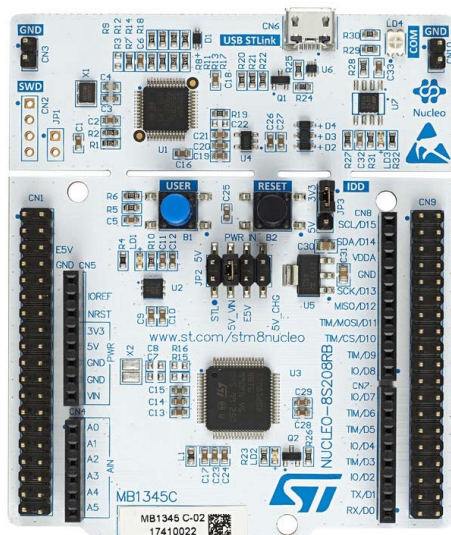
Top view of the NUCLEO-8S208RB board.
