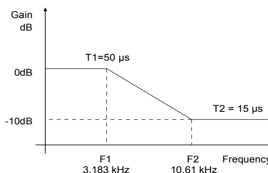
Figure 17. De-Emphasis Curve
