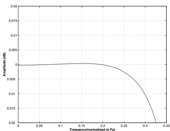
Figure 35. Double-Speed (slow) Passband Ripple
