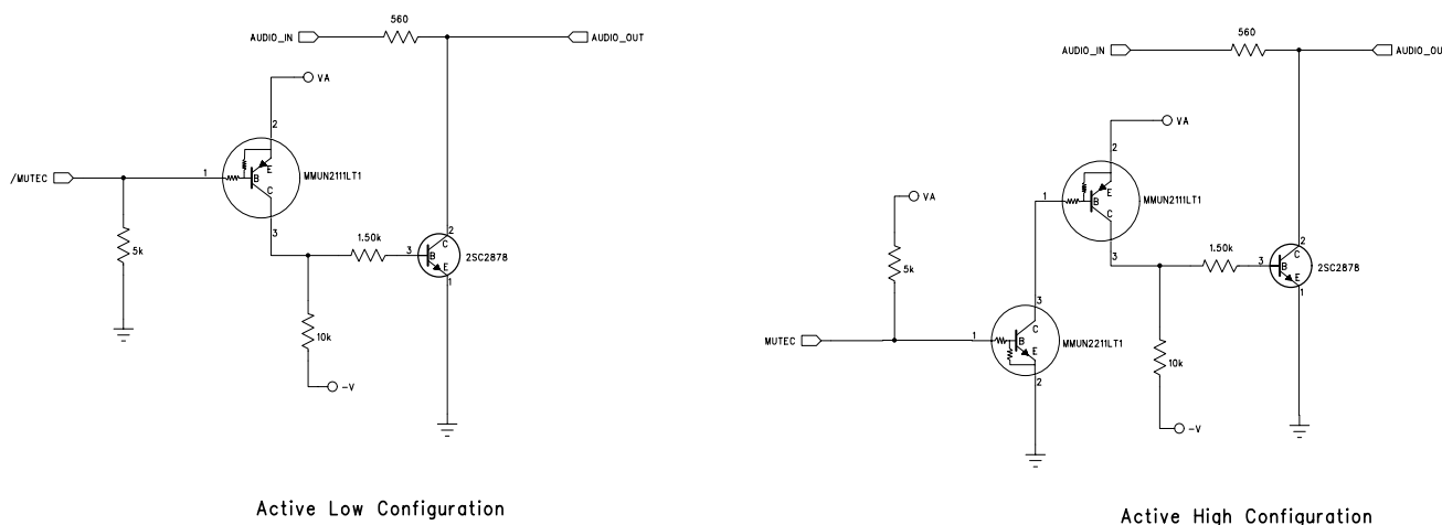
Figure 12. Recommended Mute Circuitry
