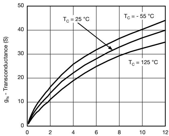
Transconductance
