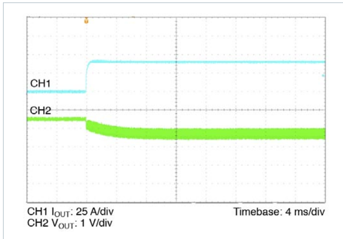
Figure 13 — 10% to 100% load transient response, V_{IN} = 290\text{ V} , nominal trim, C_{OUT\_EXT} = 1000\text{ }\mu\text{F}
