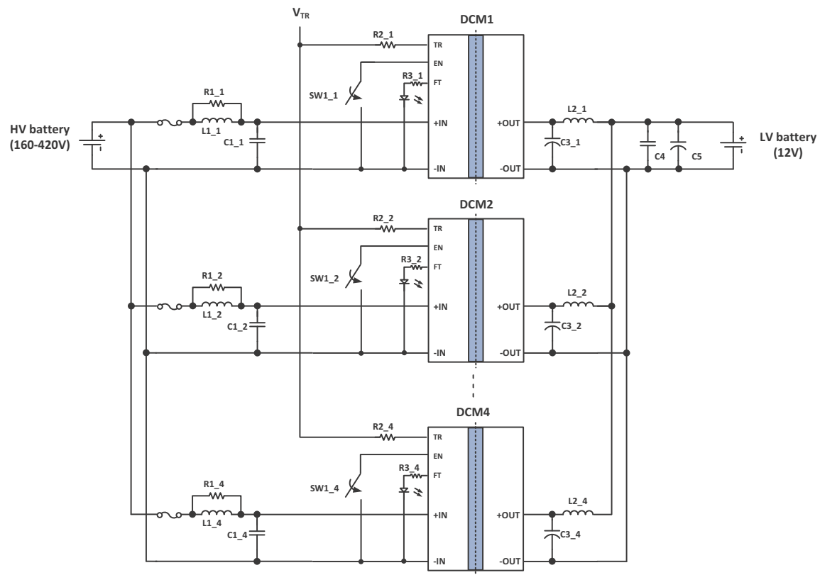
Typical Application 1: DCM290P138T600A40 for EV/HEV applications
