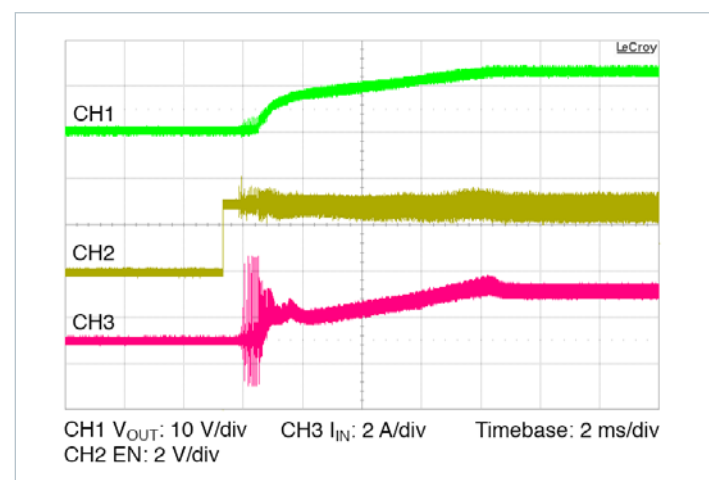
Figure 6 — Initial startup from EN pin, with soft-start ramp. V_{IN} = 290\text{ V} , C_{OUT\_EXT} = 10000\text{ }\mu\text{F} , R_{LOAD} = 0.317\text{ }\Omega
