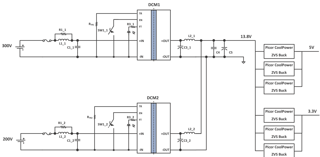
Typical Application 2: DCM290P138T600A40 + Picor Point-of-Load
