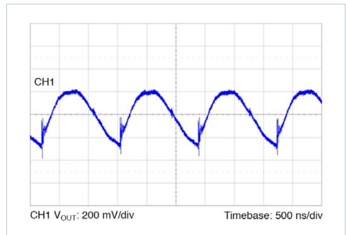
Figure 18 — Typical output voltage ripple, V_{IN} = 290\text{ V} , V_{OUT} = 13.8\text{ V} , C_{OUT\_EXT} = 1000\text{ }\mu\text{F} , R_{LOAD} = 0.317\text{ }\Omega
