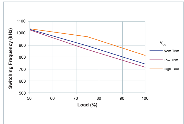
Figure 17 — Powertrain switching frequency vs. load, at nominal V_{IN}
