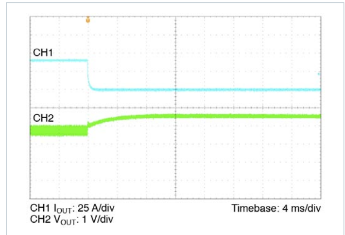
Figure 16 — 100% to 10% load transient response, V_{IN} = 290\text{ V} , nominal trim, C_{OUT\_EXT} = 1000\text{ }\mu\text{F}
