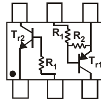
SCHMATIC DIAGRAM
