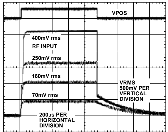
Figure 32. Output Response to Gating on Power Supply for Various RF Input Levels, Supply 3 V, Modulation Frequency 900 MHz, 0.01 μF Filter Capacitor
