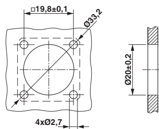
M12 flush-type plug, square flange
