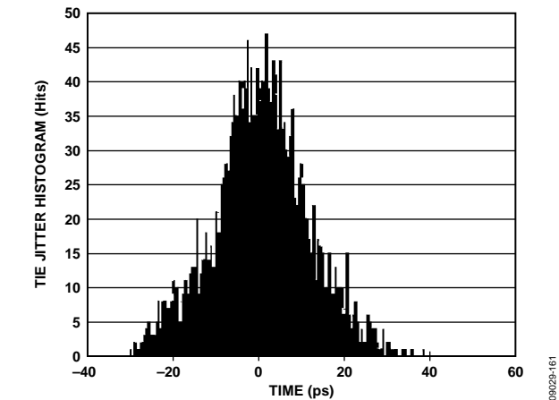
Figure 66. Data Eye for LVDS Outputs in ANSI-644 Mode with 18-Inch Trace Lengths on Standard FR-4, AD9467-250
