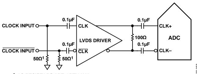
Figure 60. Differential LVDS Sample Clock
