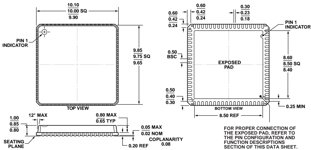
Figure 70. 72-Lead Lead Frame Chip Scale Package, Exposed Pad [LFCSP_VQ] 10 mm × 10 mm Body, Very Thin Quad (CP-72-5) Dimensions shown in millimeters
