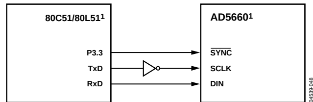
Figure 48. AD5660-to-80C51/80L51 Interface
