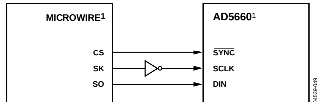
Figure 49. AD5660-to-MICROWIRE Interface
