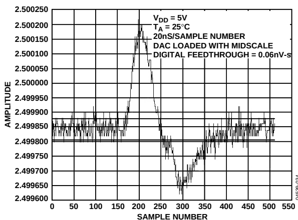
Figure 34. Digital Feedthrough
