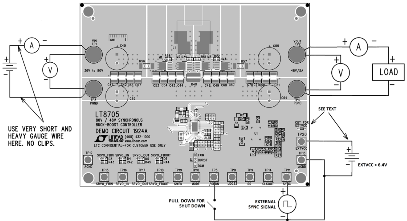
Figure 2. Test Setup
